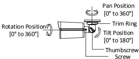
Figure 2-10 3-Axis Adjustment
